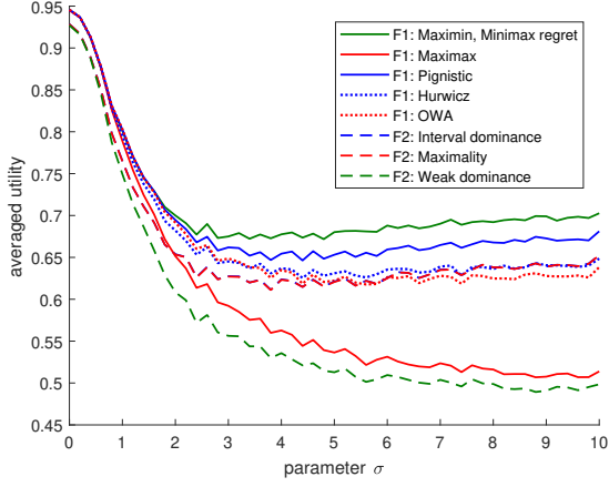
Figure 3: Averaged utilities of different criteria as a function of noise level
