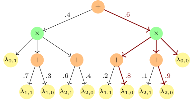
Figure 1: Selective Sum-Product Network over three binary variables.
